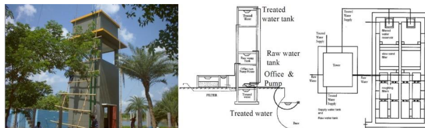
Fig. 19-5. Water tank and design
