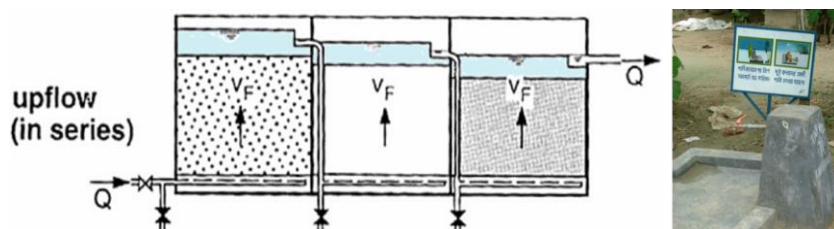
Fig. 19-4. Series of URF and public tap
