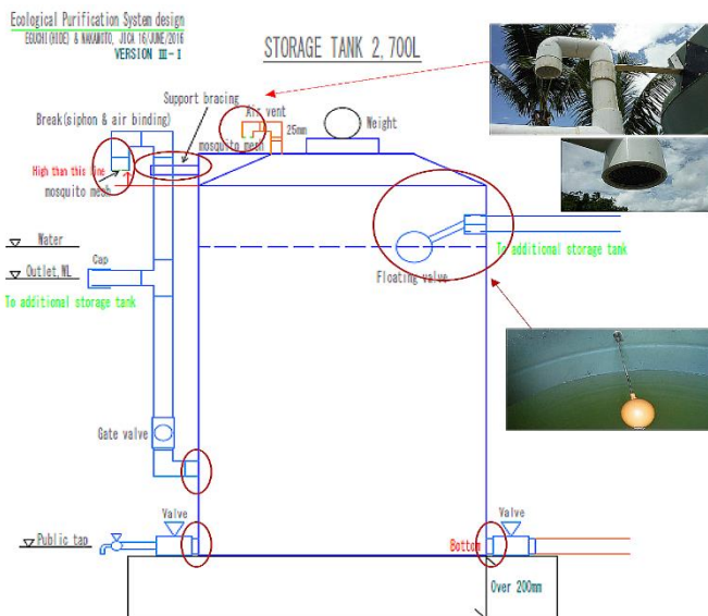
Fig. 17-15. Construction guide of Storage Tank
