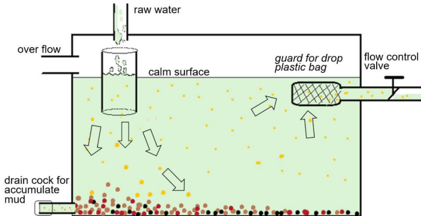
Fig. 15-8. Receiving tank (settling tank)
