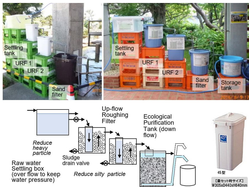
Fig. 15-5. EPS model
